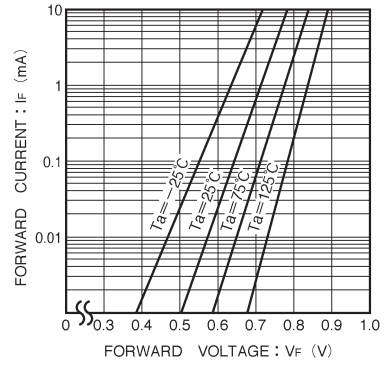
Fig. 3 Forward characteristics
