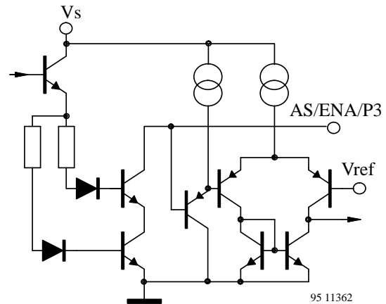
Figure 12. Address select/ Enable input
