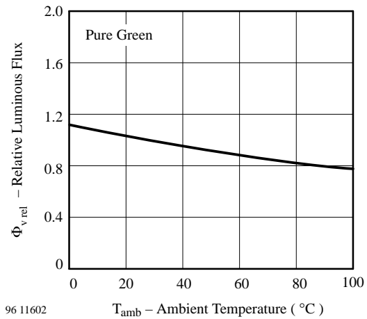
Figure 26. Rel. Luminous Flux vs. Ambient Temperature
