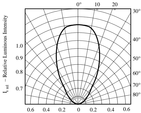
Figure 31. Rel. Luminous Intensity vs. Angular Displacement
