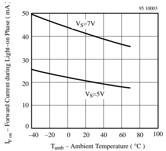
Figure 4. Forward Current (Light On) vs. Amb. Temperature
