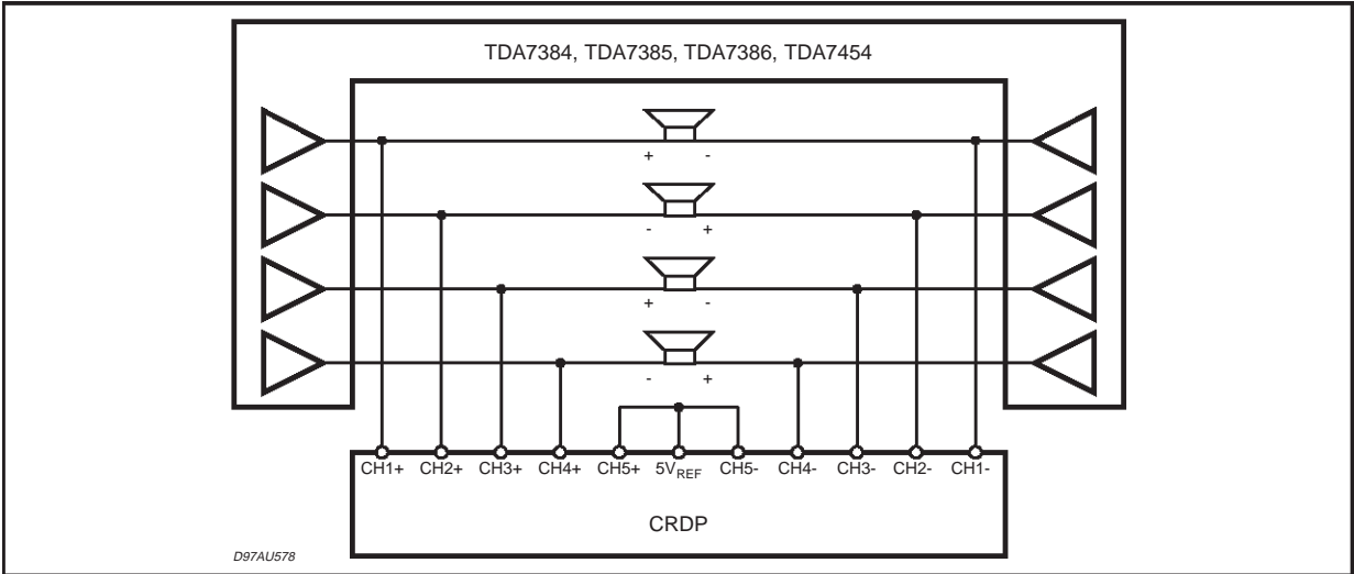
Figure 8: Quad Bridge Amplifiers
