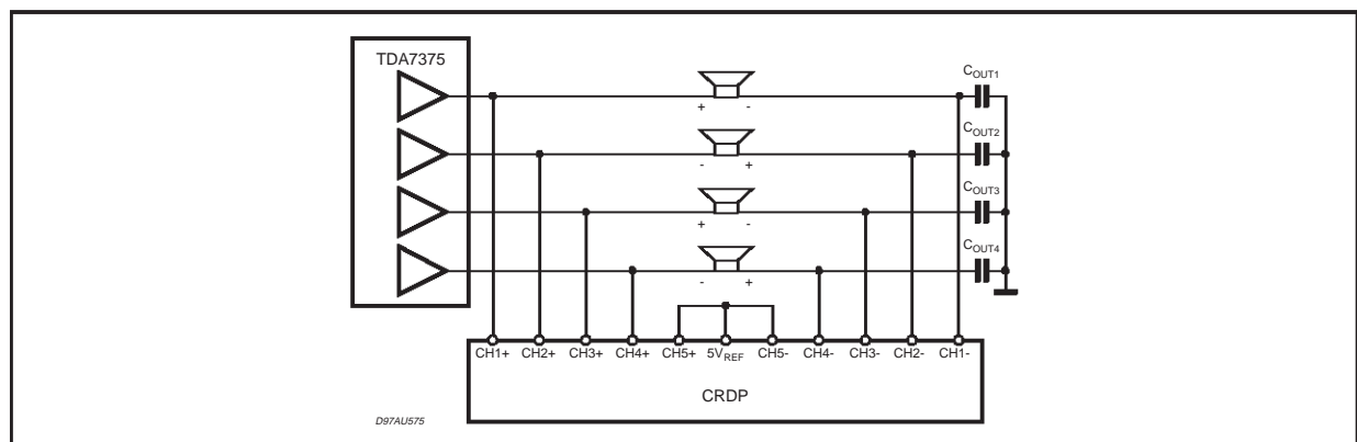
Figure 5: TDA7375 in S.E. mode with 4 output capacitors
