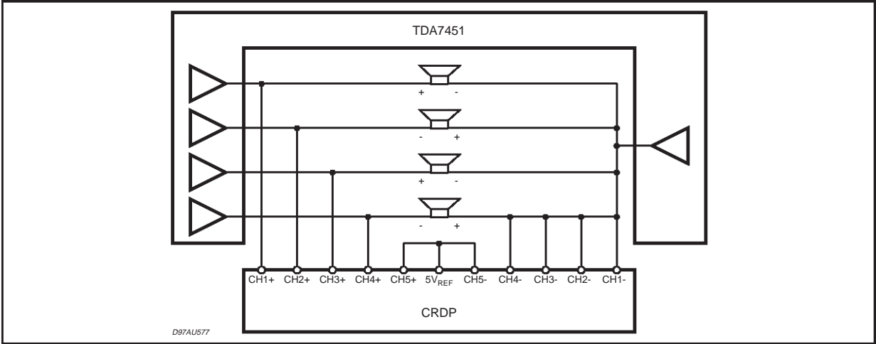
Figure 8: Quad Bridge Amplifiers
