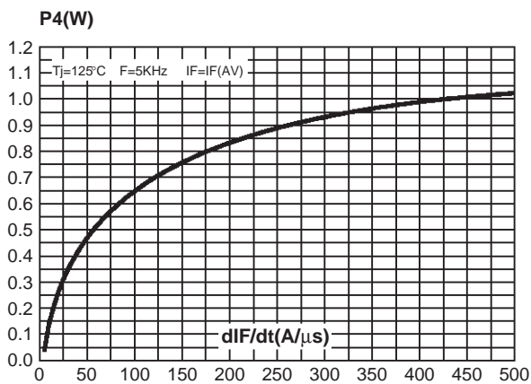
Fig. 11: Switching ON losses versus dIF/dt .
