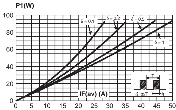
Fig. 9: Conduction losses versus average current (per diode).
