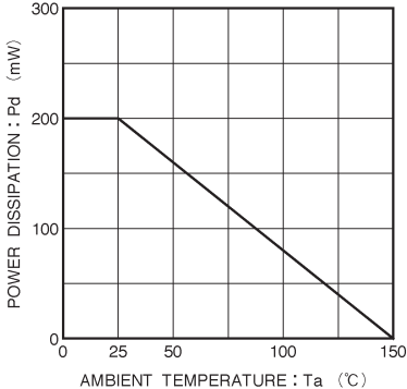
Fig. 1 Derating curve
