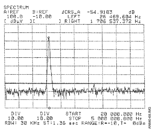
Figure 68 : I_REC = 10mA p-pk
