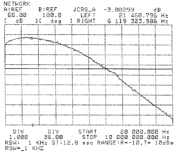
Figure 57 : H1
