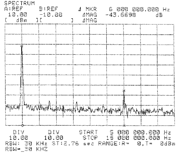
Figure 24 : Z = 470\Omega//100\text{pF}
