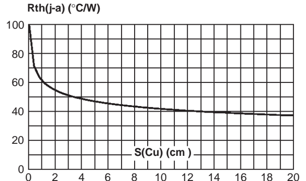
Fig. 8-3: Thermal resistance junction to ambient versus copper surface under tab (Epoxy printed circuit board FR4, copper thickness: 35\mu\text{m} ) (DPAK).
