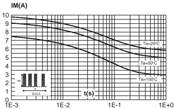
Fig. 3-1: Non repetitive surge peak forward current versus overload duration (SMB) (Maximum values).
