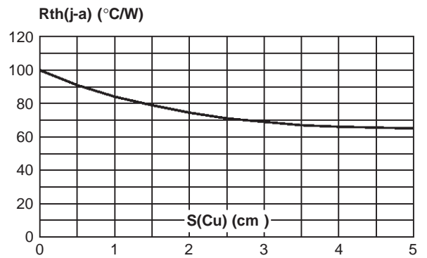
Fig. 8-1: Thermal resistance junction to ambient versus copper surface under tab (Epoxy printed circuit board FR4, copper thickness: 35\mu\text{m} ) (SMB).
