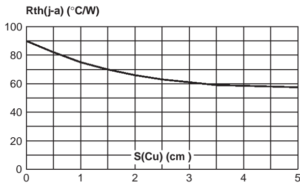
Fig. 8-2: Thermal resistance junction to ambient versus copper surface under tab (Epoxy printed circuit board FR4, copper thickness: 35\mu\text{m} ) (SMC).
