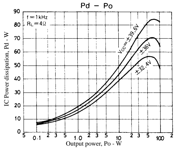
Figure 2. STK4040V Pd - Po ( R_L = 4\Omega )
