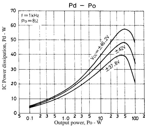
Figure 1. STK4040V Pd - Po ( R_L = 8\Omega )
