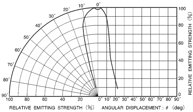
Fig. 7 Directional pattern
