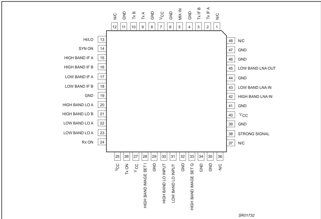
Figure 1. Pin Configuration
