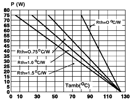
Fig. 2 : Correlation between maximum RMS power dissipation and maximum allowable temperature (Tamb) for different thermal resistances heatsink + contact.
