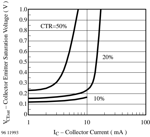
Figure 8. Collector Emitter Sat. Voltage vs. Collector Current
