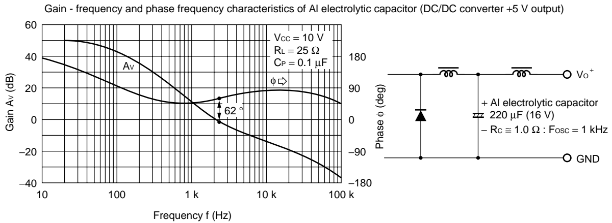
• Figure 6 Phase-Frequency characteristic
