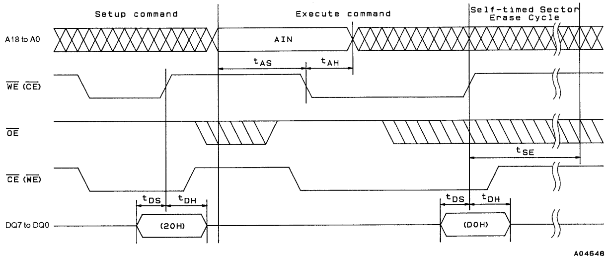
Figure 6 Sector Erase
