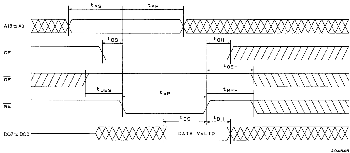
Figure 4 WE Control Write Cycle
