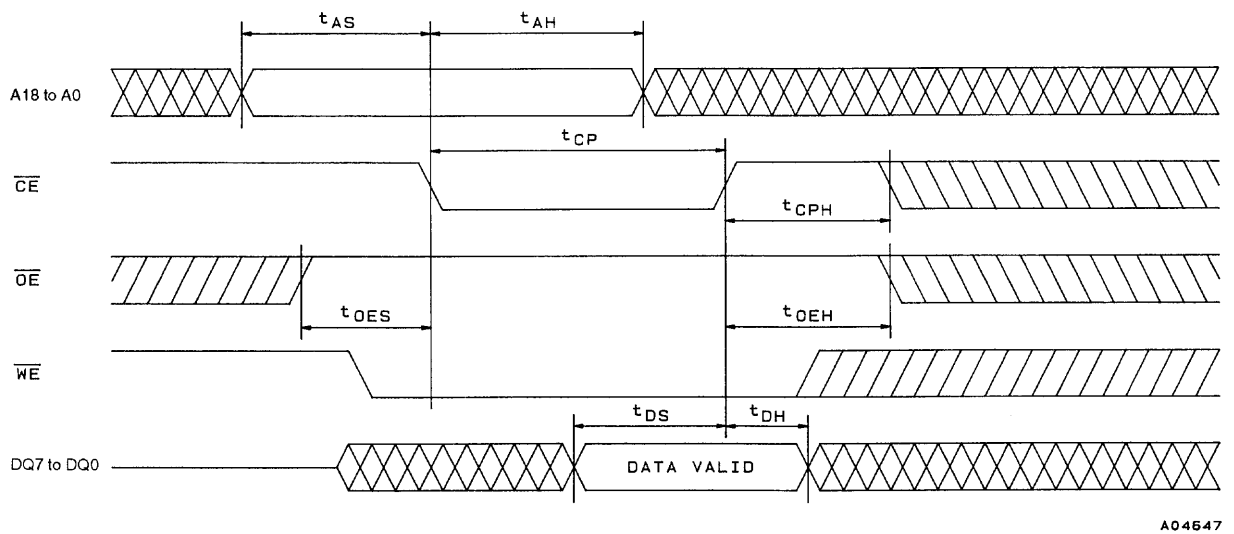
Figure 5 CE Control Write Cycle
