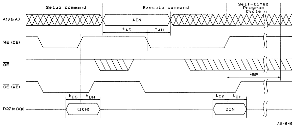
Figure 7 Byte Programming
