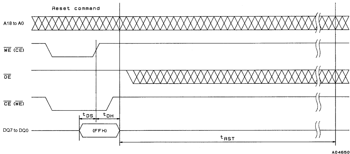
Figure 8 Reset
