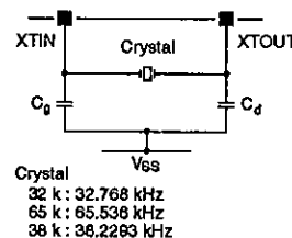
Figure 8. Crystal oscillator
