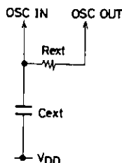
Fig.11 Recommended CR oscillation circuit
