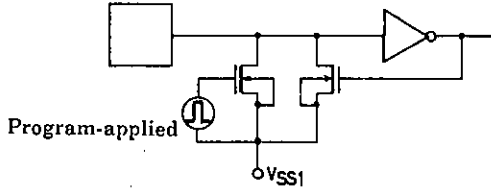
Fig.1 Input configuration of S1-4, M1-4
