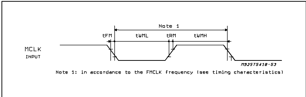
Figure 27: MCLK ALL MODES
