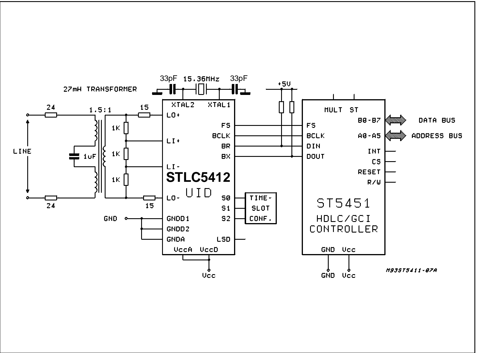
Figure 13a: LT Application.
