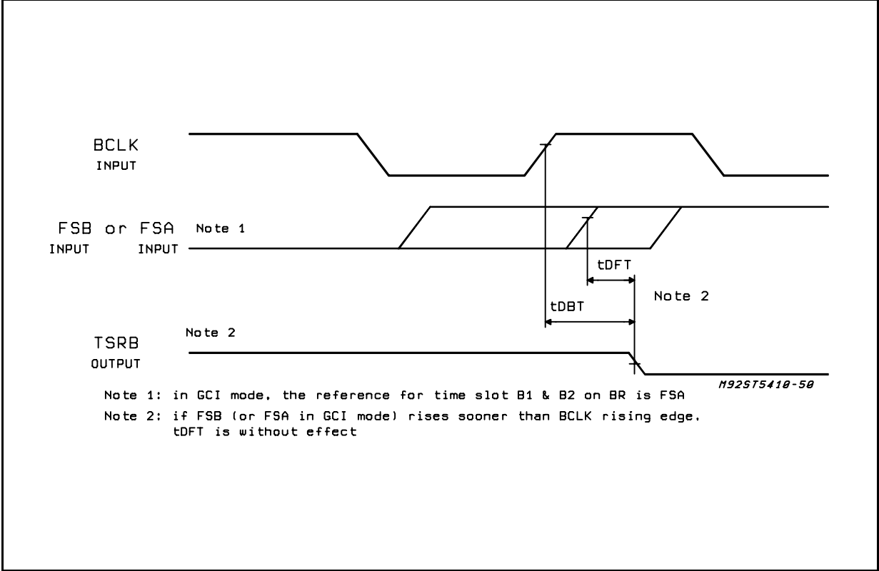
Figure 25: SPECIAL CASE TSRB, B1 OR B2 FIRST CHANNEL OF THE FRAME, IN SLAVE & NON DELAYED MODE, FORMATS 1 3 (MW MODE), FORMAT 4 (μW & GCI MODE)
