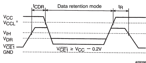
Data Retention Waveforms (1): CE1 Control
