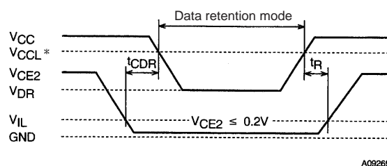
Data Retention Waveforms (2): CE2 Control
