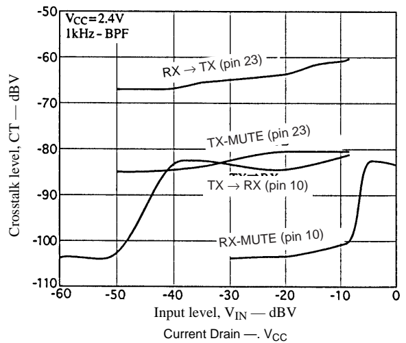
Crosstalk Characteristics
