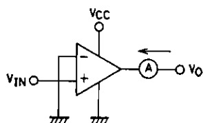
9. Output leak current
