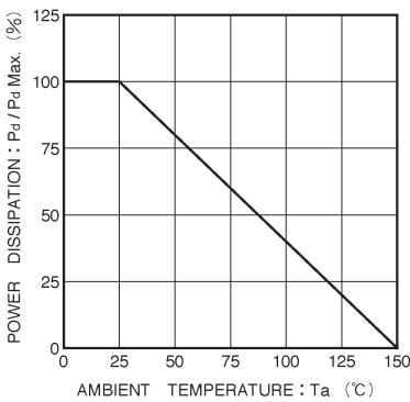
Fig. 1 Derating curve (mounting on glass epoxy PCBs)
