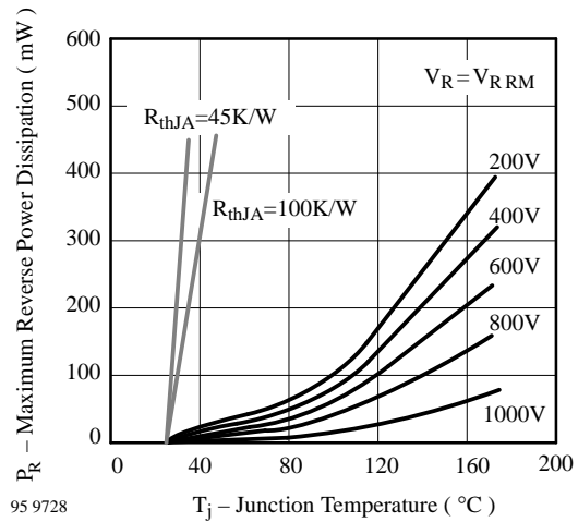
Figure 2. Maximum Reverse Power Dissipation vs. Junction Temperature
