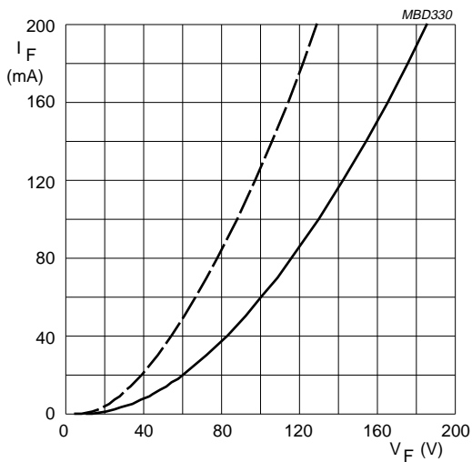
BY8420. Dotted line: T_j = 120^\circ\text{C} . Solid line: T_j = 25^\circ\text{C} .
