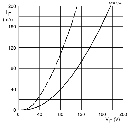
BY8418. Dotted line: T_j = 120^\circ\text{C} . Solid line: T_j = 25^\circ\text{C} .
