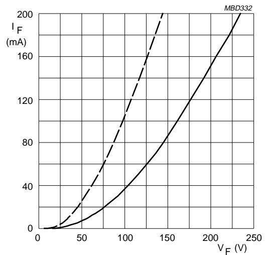
BY8424. Dotted line: T_j = 120^\circ\text{C} . Solid line: T_j = 25^\circ\text{C} .
