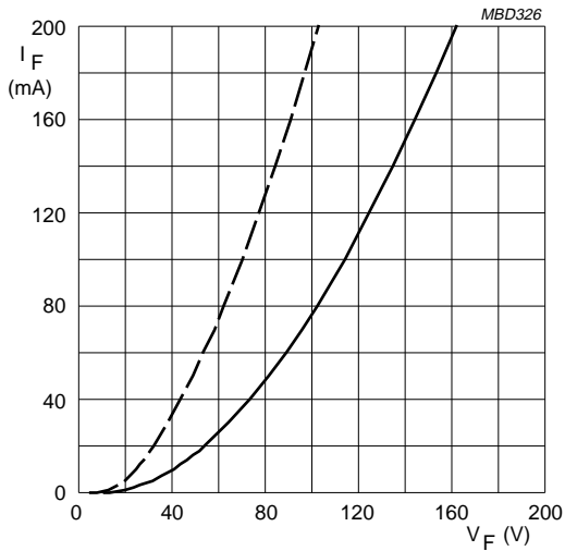
BY8416. Dotted line: T_j = 120^\circ\text{C} . Solid line: T_j = 25^\circ\text{C} .
