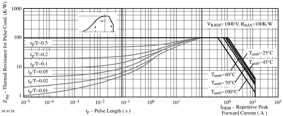
Figure 8. Thermal Response
