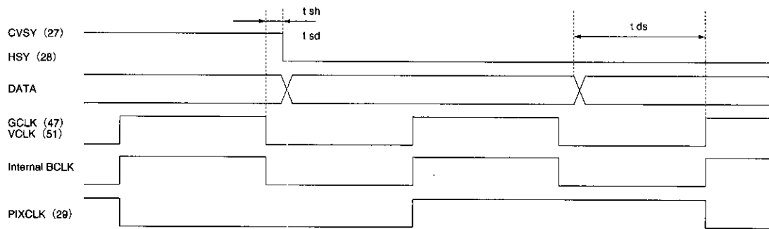
Fig. 8 Clock timing and data input timing
