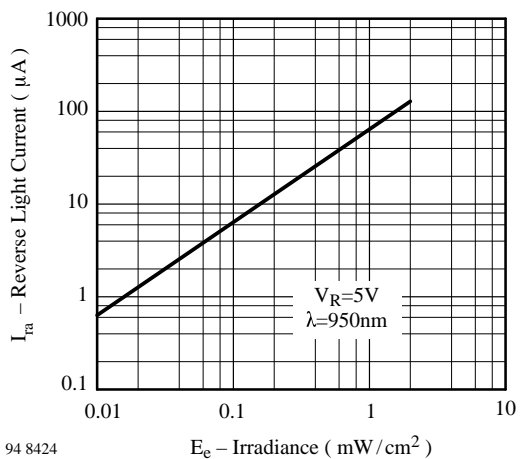
94 8424 E_c – Irradiance ( \text{mW}/\text{cm}^2 ) Figure 3. Reverse Light Current vs. Irradiance
