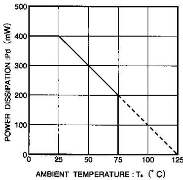
Fig.20 Power dissipation curve
