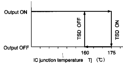
Fig.2 Thermal shutdown characteristic
