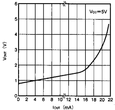
Fig. 4 CTL amplifier sink current vs. output voltage
