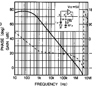
Fig. 2 CTL amplifier frequency characteristics
