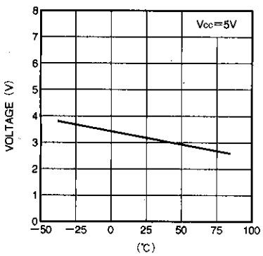
Fig. 7 Pin 2 DC bias voltage temperature characteristics
