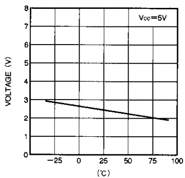
Fig. 8 Pin 3 bias voltage temperature characteristics
