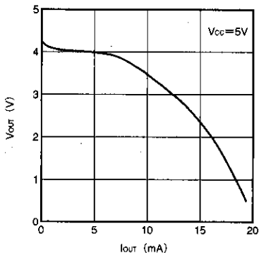
Fig. 5 FG amplifier source current vs. output voltage
