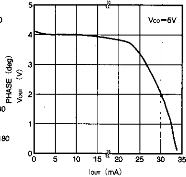
Fig. 3 CTL amplifier source current vs. output voltage
