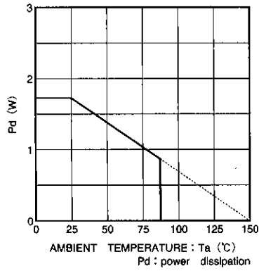
Fig. 4 When mounted to a 50×50×1.0 (mm) paper phenol board Pd : power dissipation
