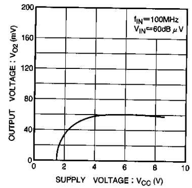
Fig. 5 Output voltage 2 vs. supply voltage
