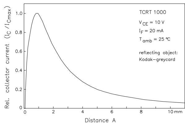
d) TCRT1000
