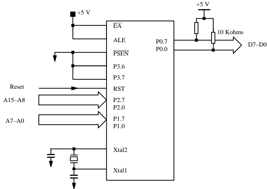
Figure 1. Configuration for the TEST MODE VER
