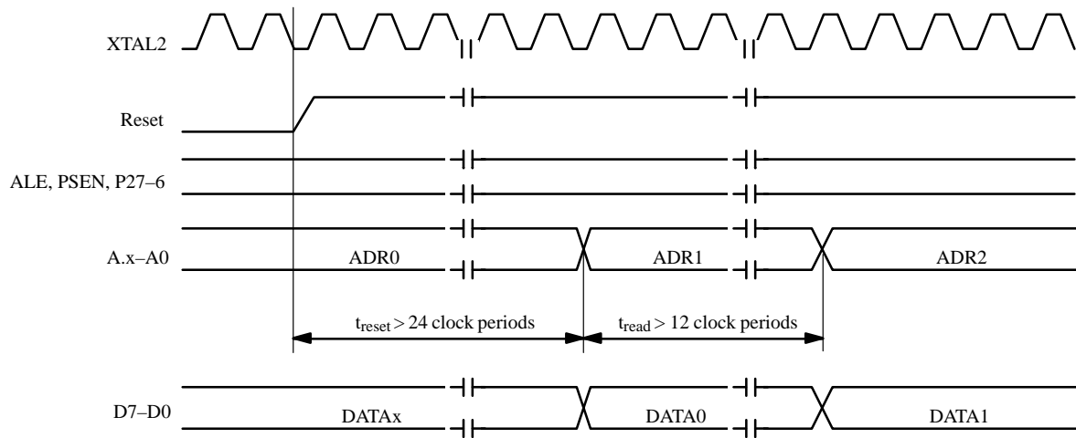
Figure 2. Timings to dump the ROM
