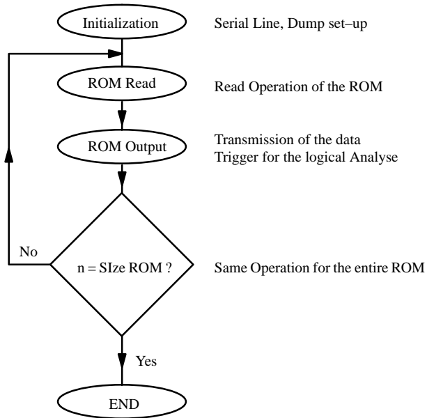
Figure 4. Flow chart for the dump ROM program
