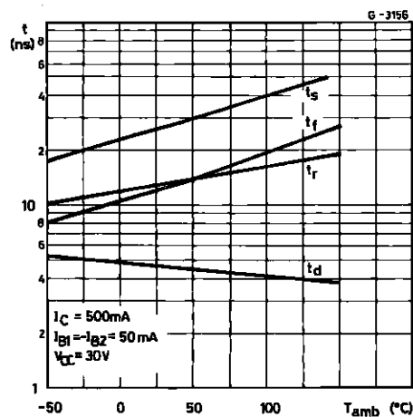
Switching Characteristics.
