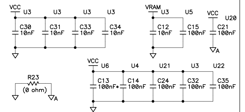
Decoupling Capacitors
