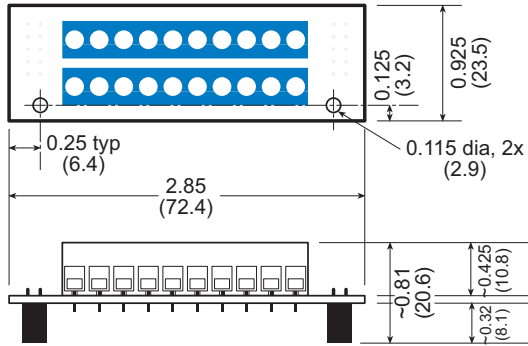
Figure C-4. FWT50 Dimensions
