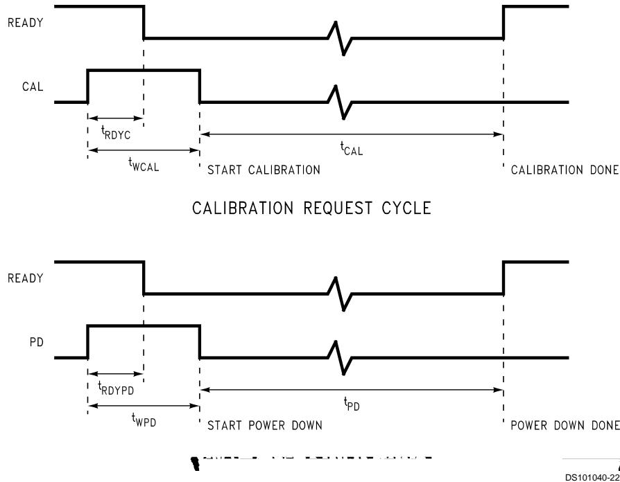
FIGURE 4. Reset and Calibration Timing
