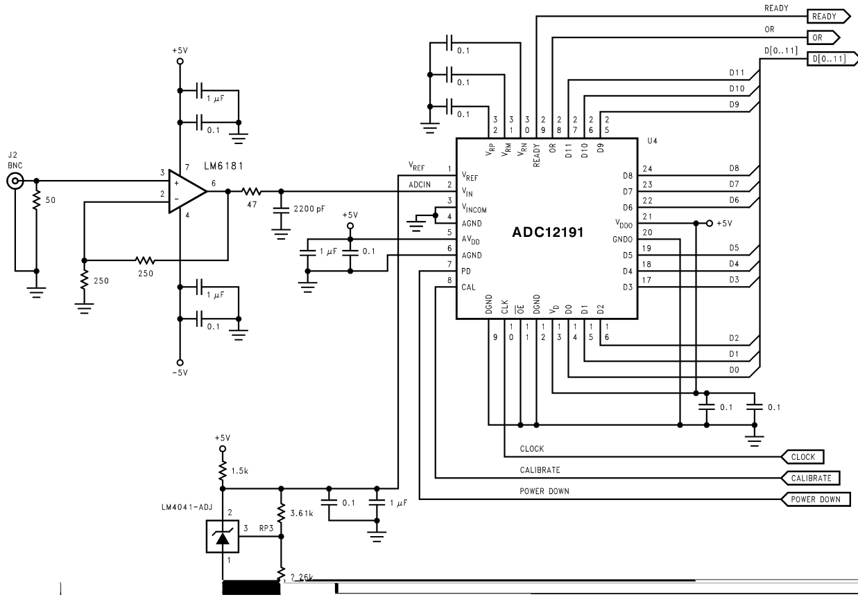
FIGURE 5. Basic Connections Diagram
