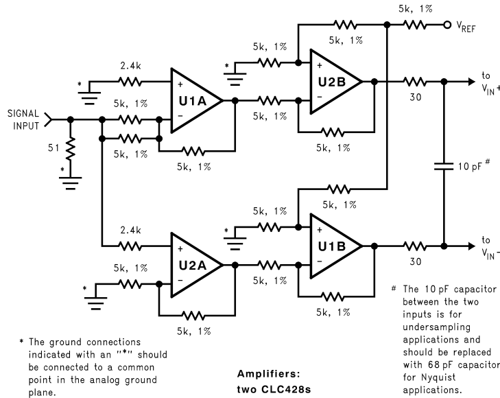
FIGURE 5. Differential Drive Circuit of Figure 4
