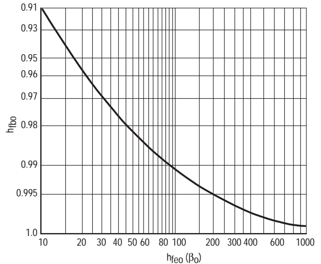
Figure 3. The Relationship Between h_{fe0} and h_{fb0} is given by the Graph Shown
