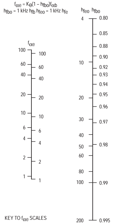
Figure 7. Once f_{\alpha b} is Known this Nomogram is Used to Find f_{\alpha e}
