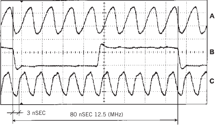
This scope photo shows some key waveforms in the circuit of Figure 1.
