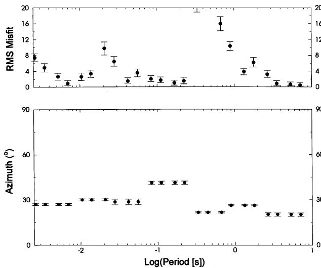
FIG. 12. Misfit error and strike azimuth from multisite decomposition for PNG sites 101–108 constrained over frequency bands of half a decade.
