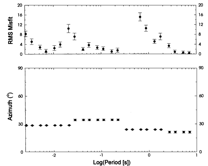
FIG. 13. Misfit error and strike azimuth from multisite decomposition for PNG sites 101–108 constrained over frequency bands of a decade.
