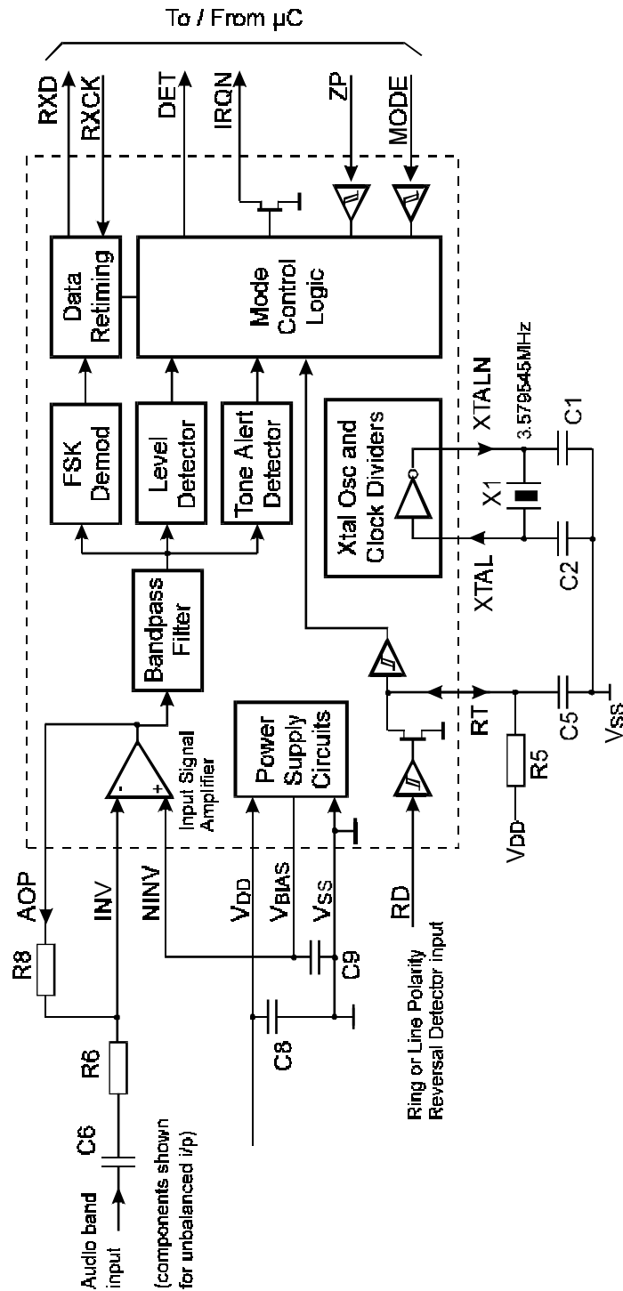
Figure 1 Block Diagram
