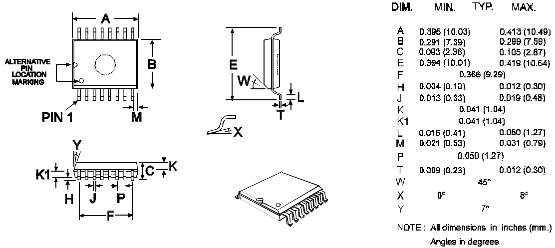
Figure 12 : 16-pin SOIC (D4) Mechanical Outline: Order as part no. FX602D4
