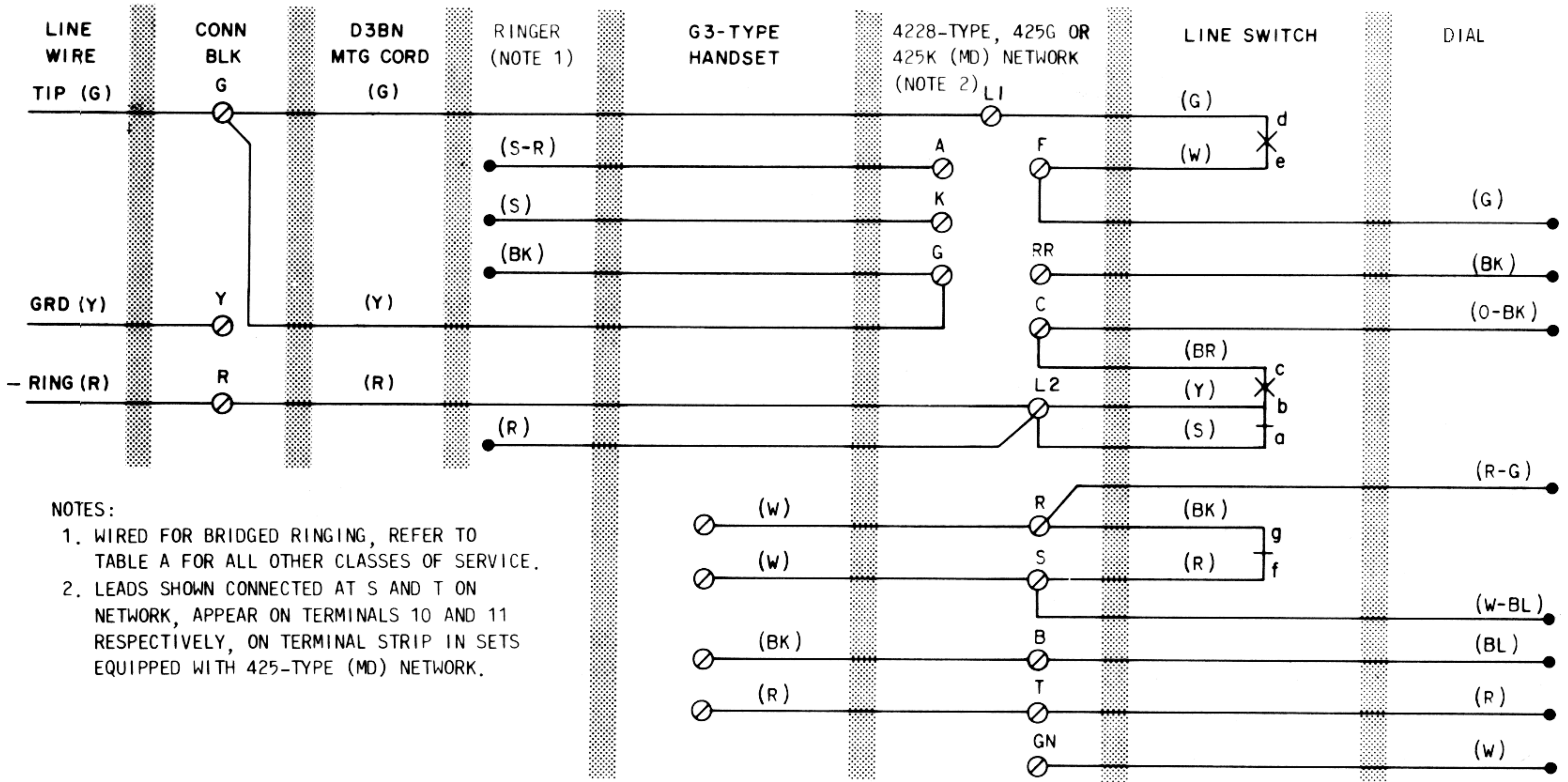
Fig. 1—2500D (MD) Telephone Set, Connections
