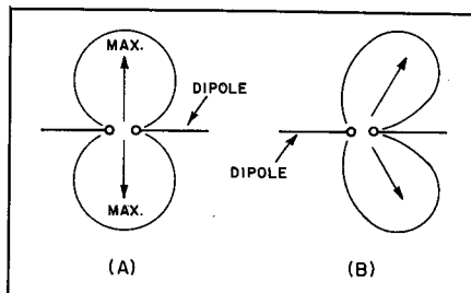
Fig. 1 — A theoretically correct radiation pattern for a half-wavelength dipole (A), and one that has a pattern skew caused by an imbalance in the feed system (B).
