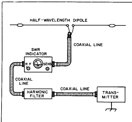
Fig. 3 — Harmonic energy from the transmitter can cause a false SWR reading. Installation of a harmonic filter, as shown here, can correct the problem.
