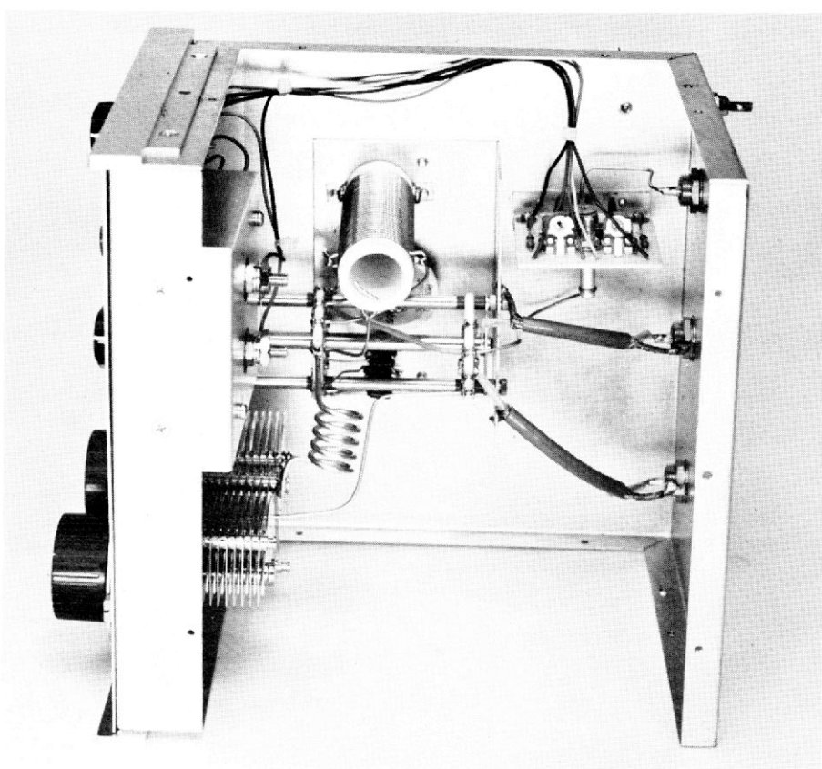
Interior view of a medium-power commercially built Transmatch. The unit shown is a Leader LAC-895. SWR-indicator circuitry is visible at the upper right. The coils and capacitors for the tuning network are at the left, along with a band switch (left center).
