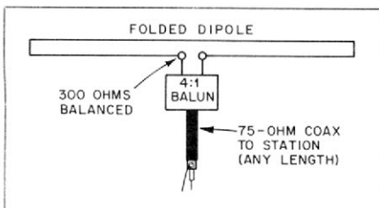
Fig. 2 — A balanced, 300-ohm, half-wave dipole can be fed with 75-ohm unbalanced line (coax) by installing a 4:1 balun transformer directly at the feed point.
