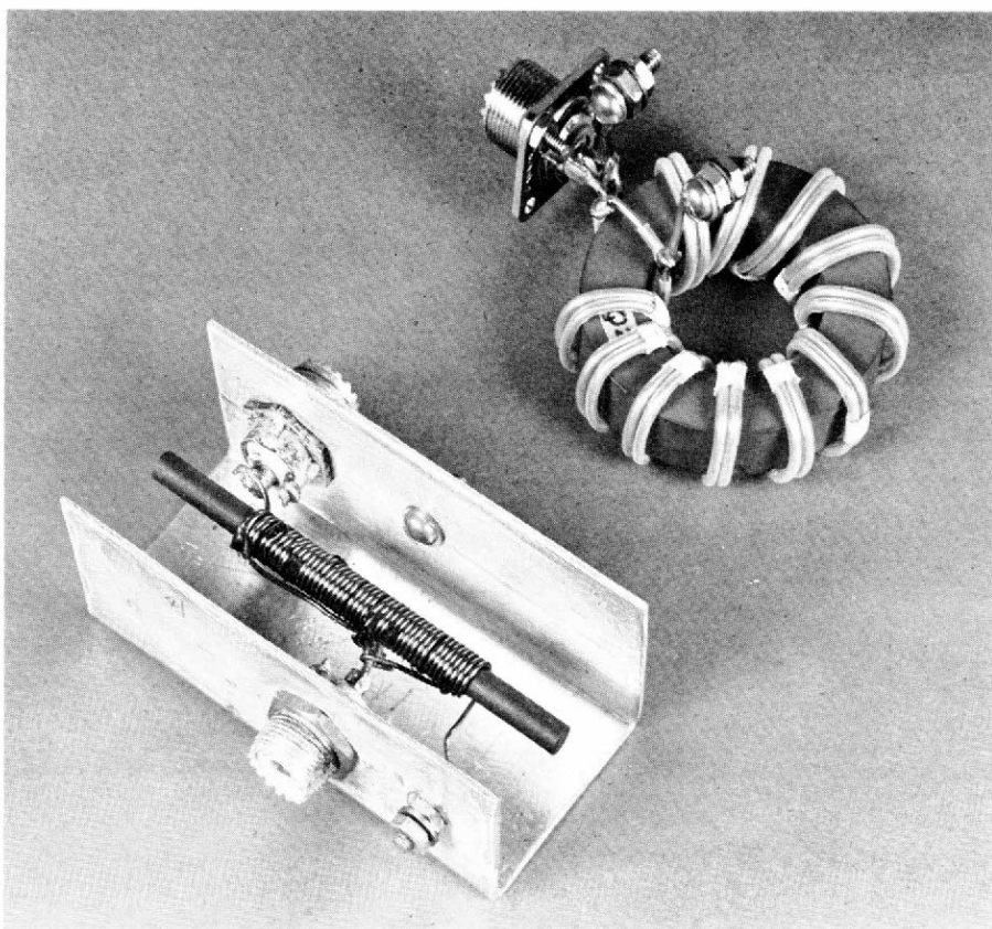
Broadband transformers of the type used as baluns. The model on the left is solenoidal. At the right is a toroidal transformer. (photo courtesy of W2FM1)
