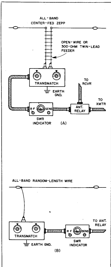
Fig. 4 — A Transmatch can be justified when it is necessary to use the same dipole on several amateur bands. The example at A shows a Transmatch connected to balanced feeders which supply power to a center-fed Zepp antenna. At B, we have a random-length wire being matched to the transmitter by means of a Transmatch to provide multiband operation. An effective earth ground is necessary to reduce the effects of rf appearing on the station equipment.
