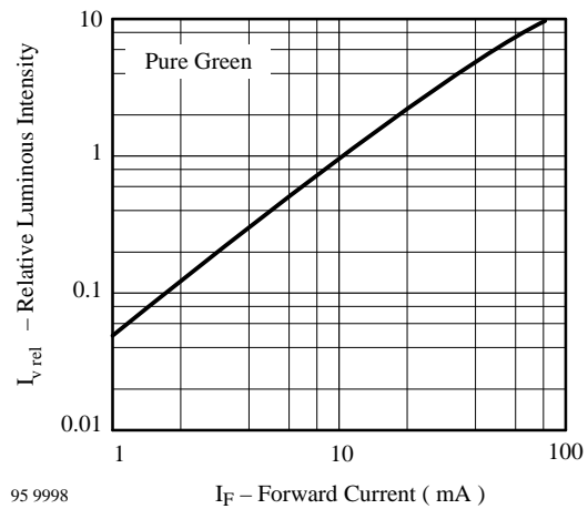
Figure 29. Relative Luminous Intensity vs. Forward Current
