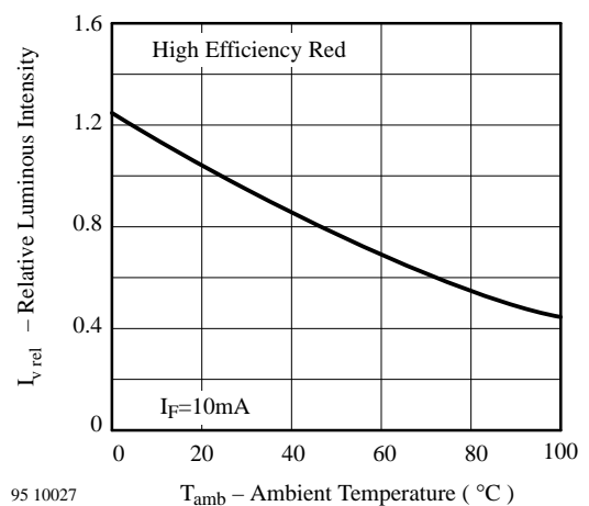
Figure 12. Rel. Luminous Intensity vs. Ambient Temperature
