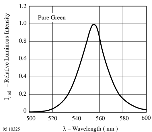
Figure 30. Relative Luminous Intensity vs. Wavelength
