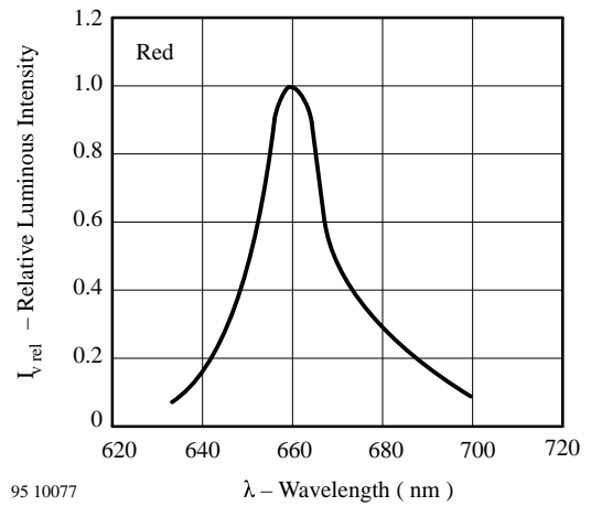
Figure 10. Relative Luminous Intensity vs. Wavelength
