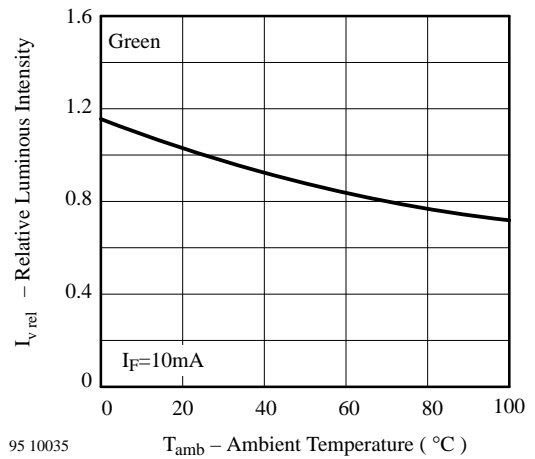
Figure 22. Rel. Luminous Intensity vs. Ambient Temperature
