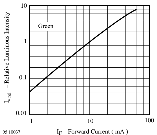
Figure 24. Relative Luminous Intensity vs. Forward Current
