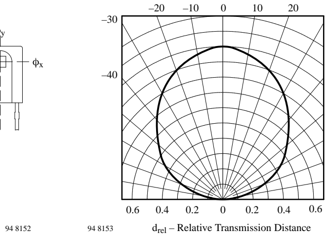
Figure 13. Horizontal Directivity \phi_x
