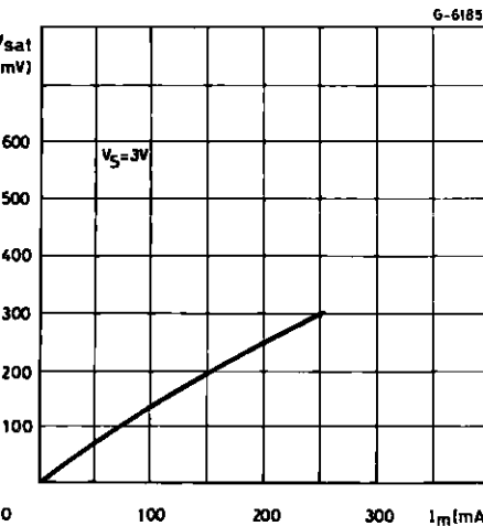
Figure 18: Saturation Voltage vs. Load Current (MOTOR)
