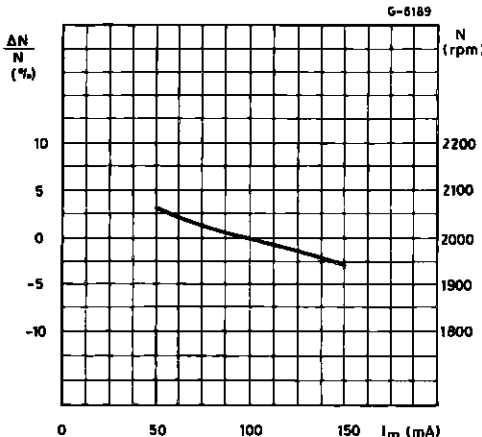
Figure 20: Speed Variations vs. Motor Current (MOTOR)
