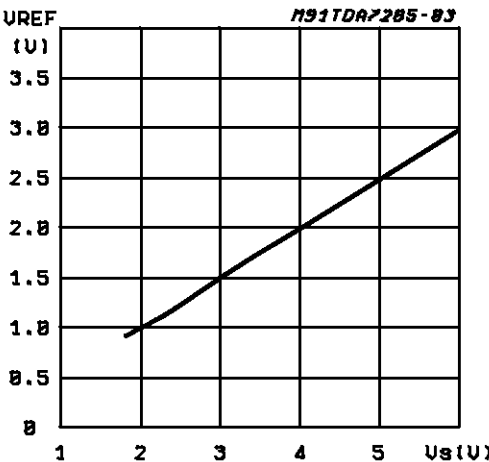
Figure 4: Reference voltage V_{S/2} (pin 20) vs. Supply Voltage
